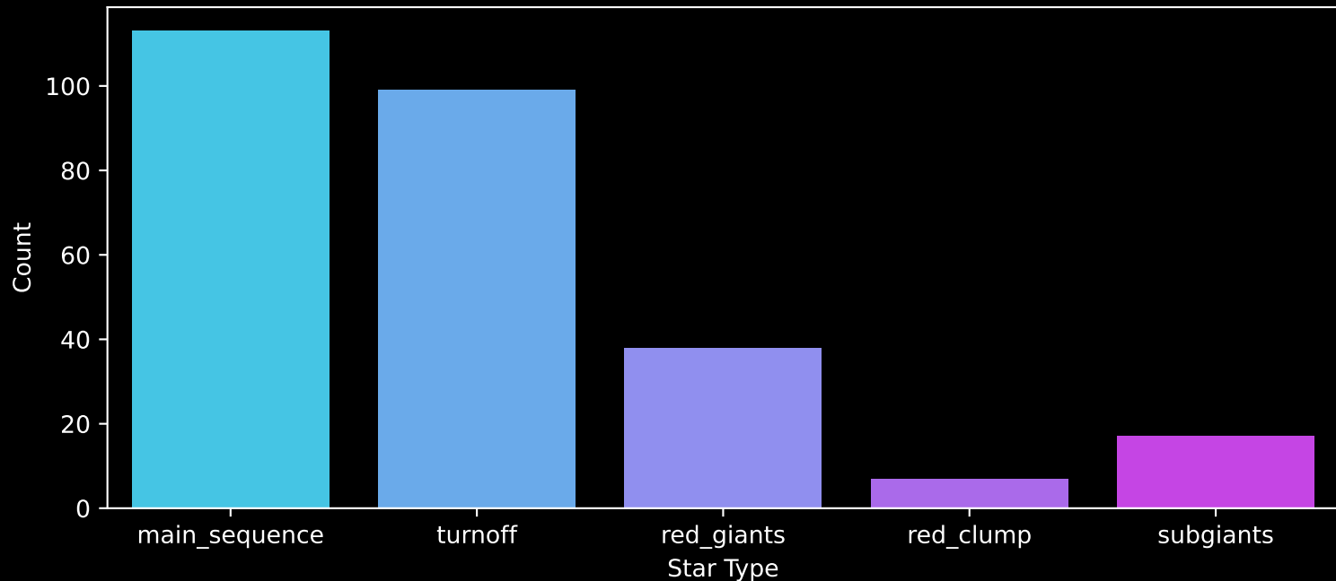
GALAH DR4 Field: [1326] Count plot of Star Type
