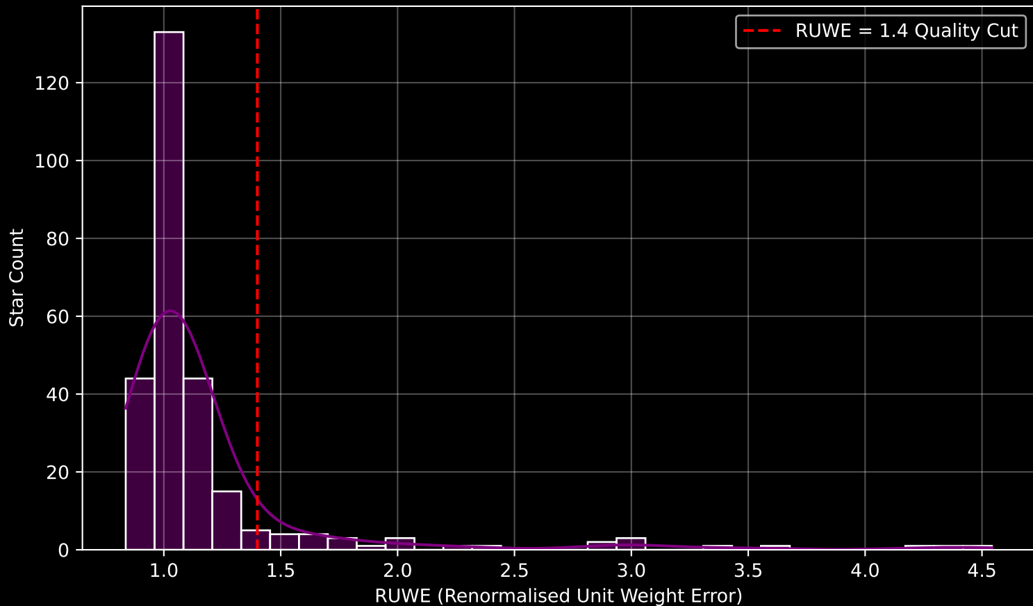
GALAH DR4 Field [1326] RUWE Distribution (n= 268)
