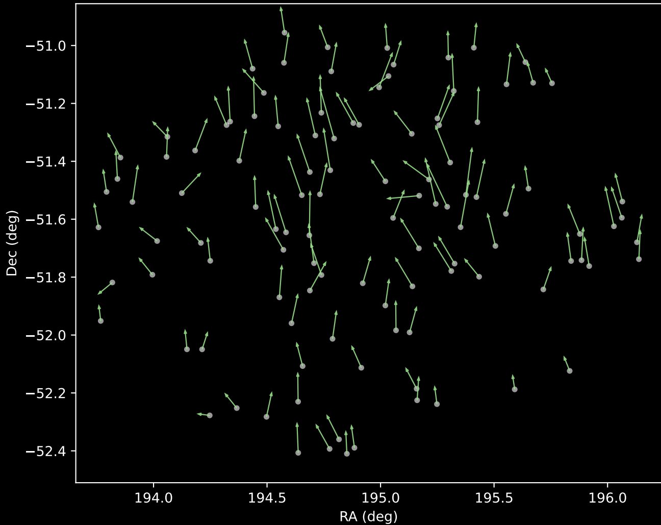
GALAH DR4 Cluster 5 Proper Motion Vectors (n=111)
