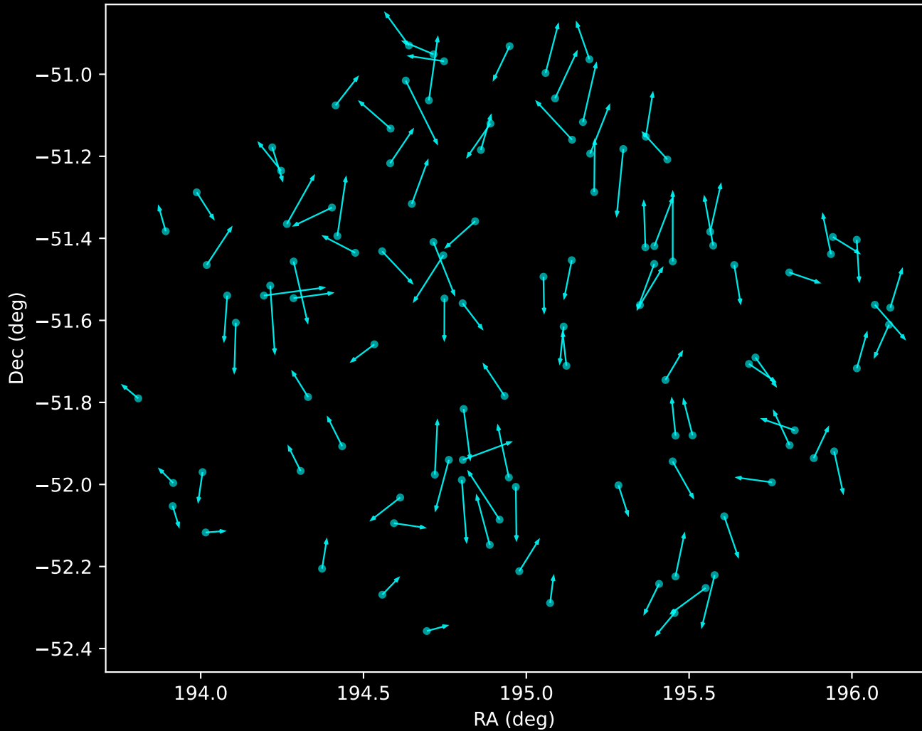
GALAH DR4 Noise Stream Proper Motion Vectors (n=107)
