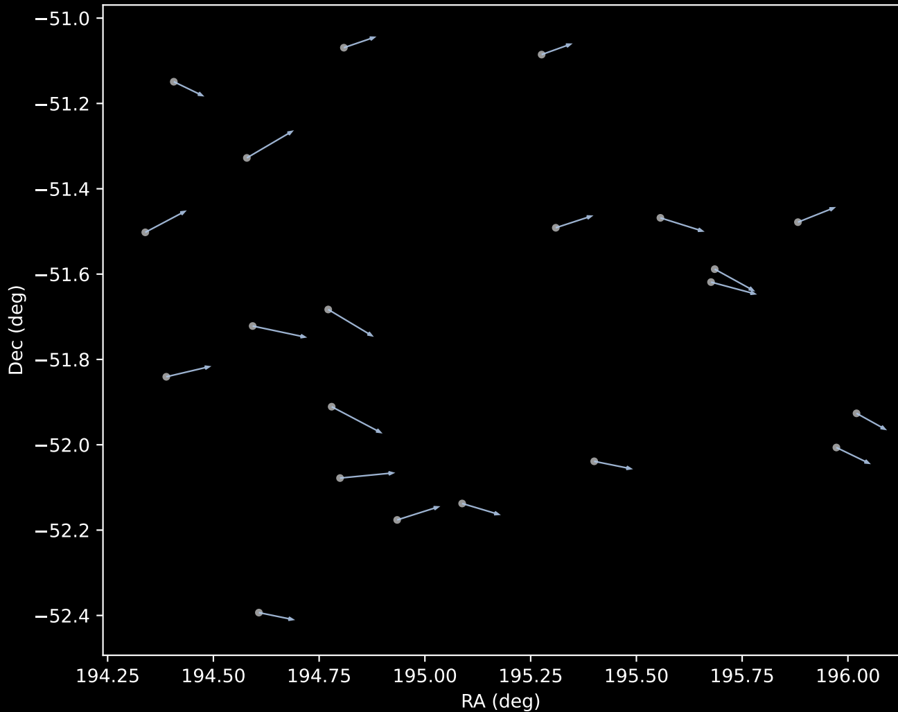
GALAH DR4 Cluster 1 Proper Motion Vectors (n=21)
