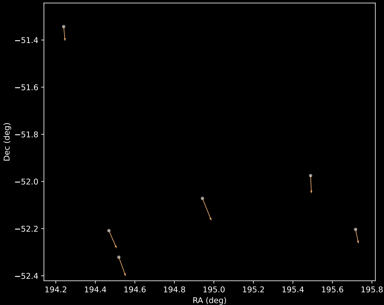
GALAH DR4 Cluster 3 Proper Motion Vectors (n=6)
